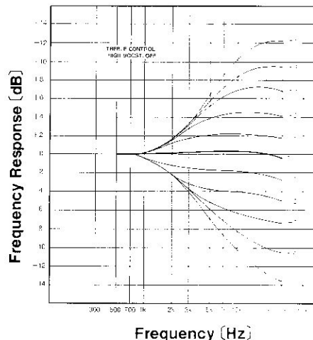
(2) Characteristics of change: tone controls⑰ and boost/filter selectors⑯ combined
