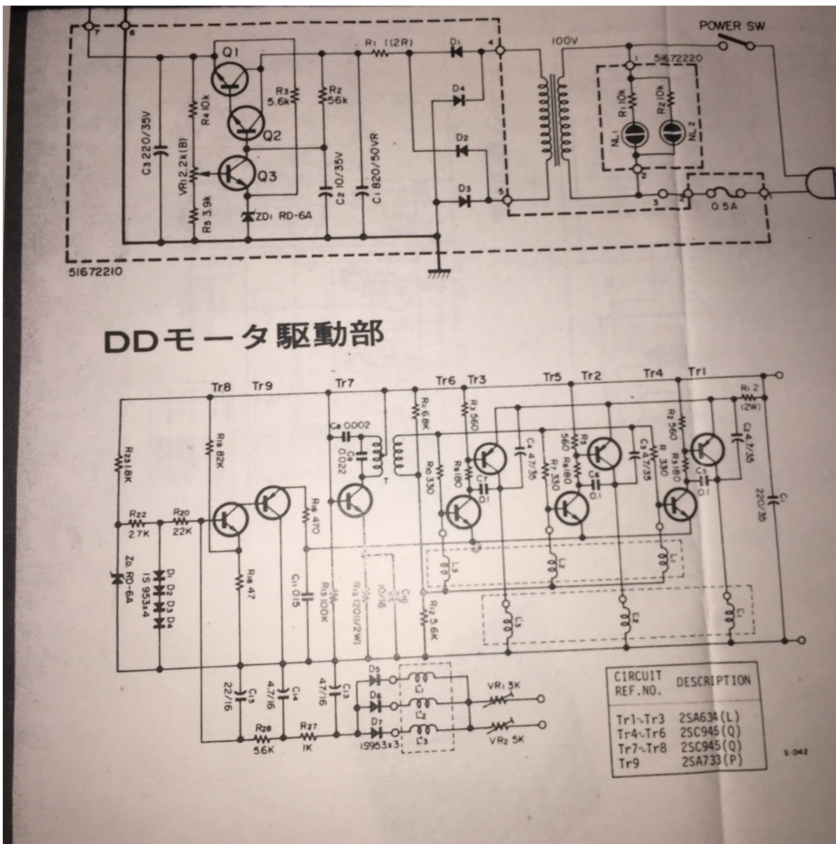
Teac TN-400 Magnefloat Turntable schematic (2 of 2)
