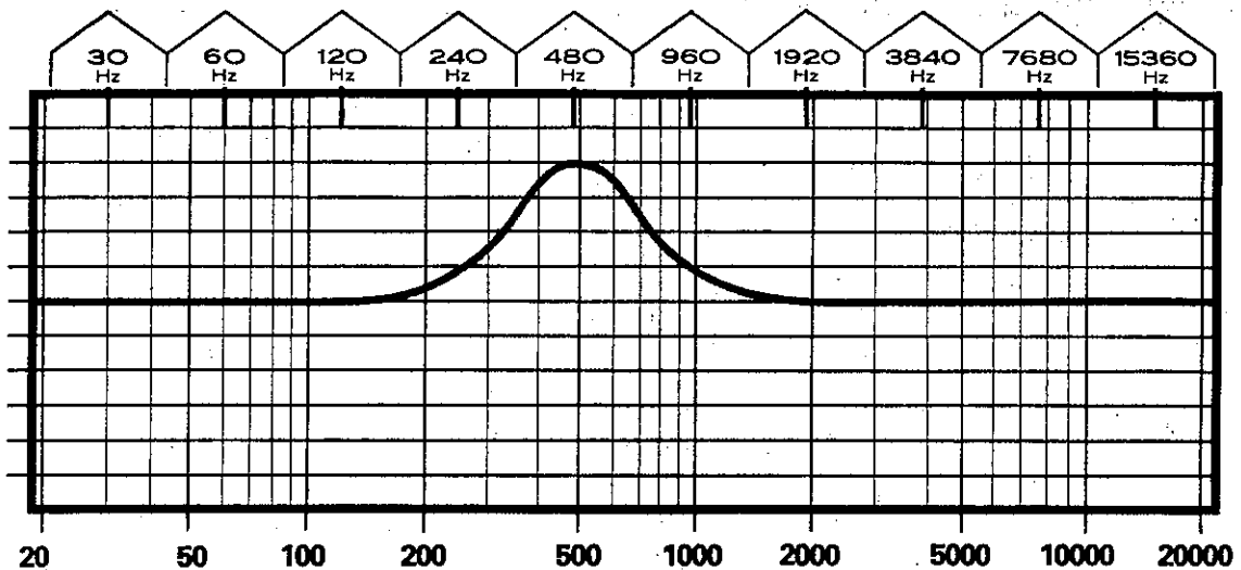
FIGURE VII FILTER SHAPE
