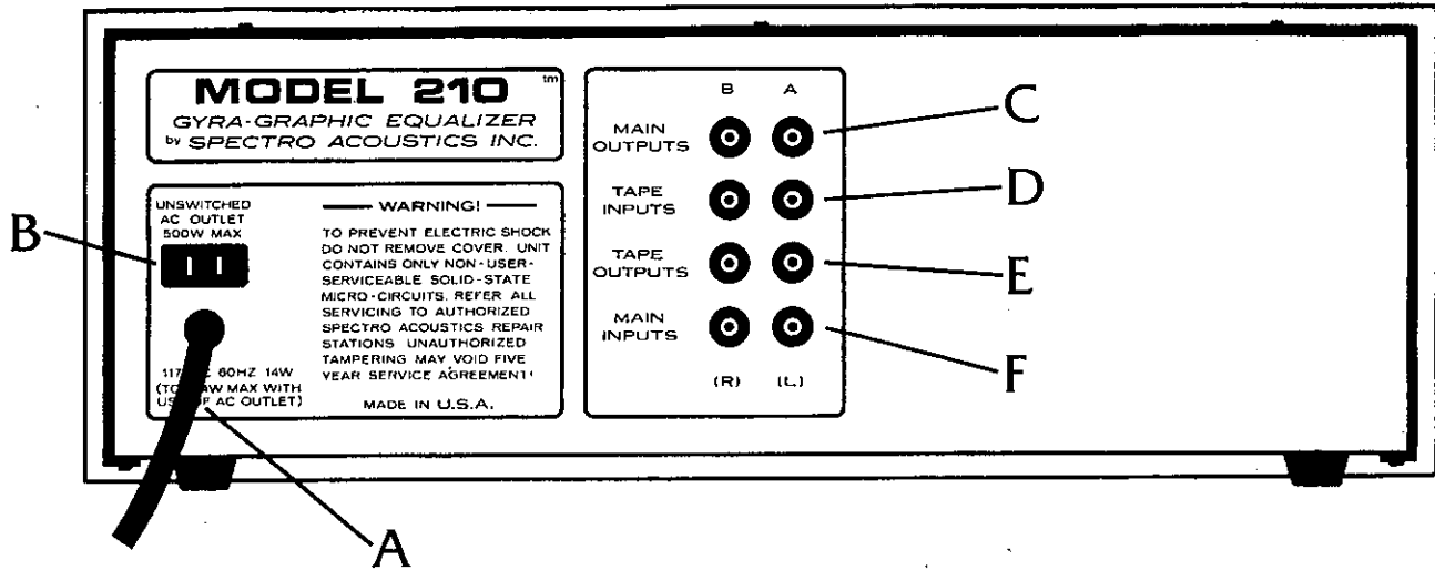
FIGURE VI REAR PANEL
