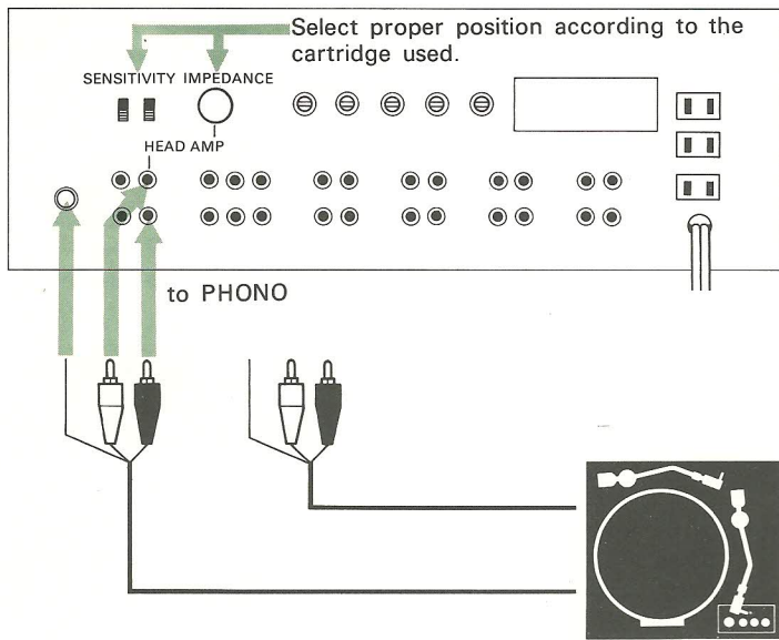
Insert the shorting plugs into the unused PHONO inputs.
