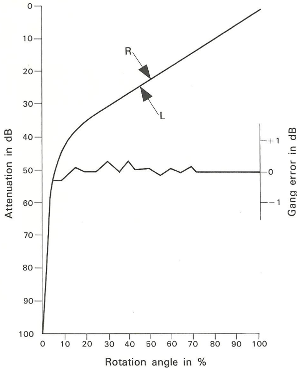
TAE-8450 Step-attenuator Volume Control
