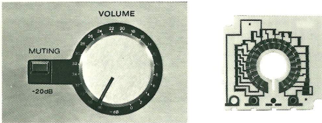
TAE-8450 Step-attenuator Volume Control
