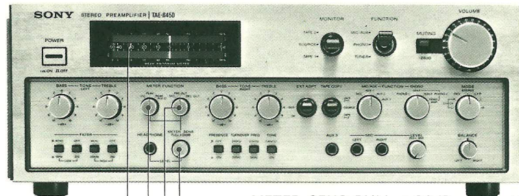
—METER SENS PULL + 20dB switch (dual function) —METER FUNCTION (right, source signal selector) —METER FUNCTION (left, meter mode selector) —The Peak Program Meters
