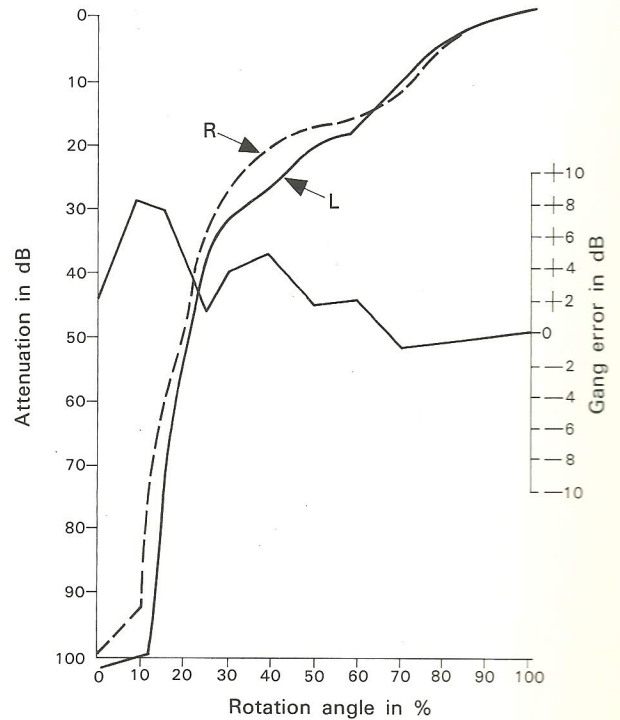
Conventional Volume Control
