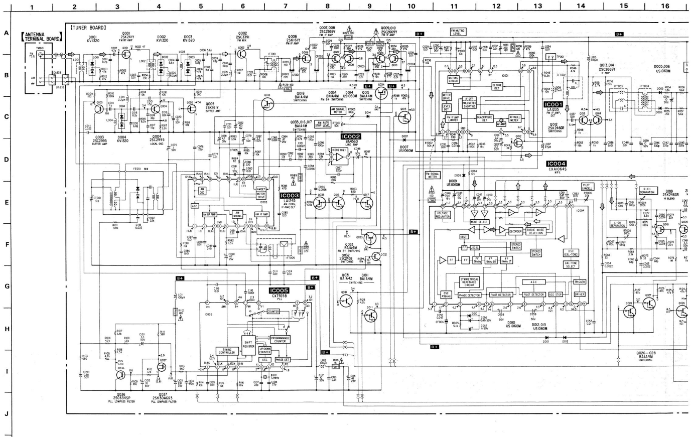
3-4. SCHEMATIC DIAGRAM —TUNER SECTION—
