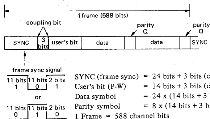
Frame Structure of EFM Modulated Recorded Signal
