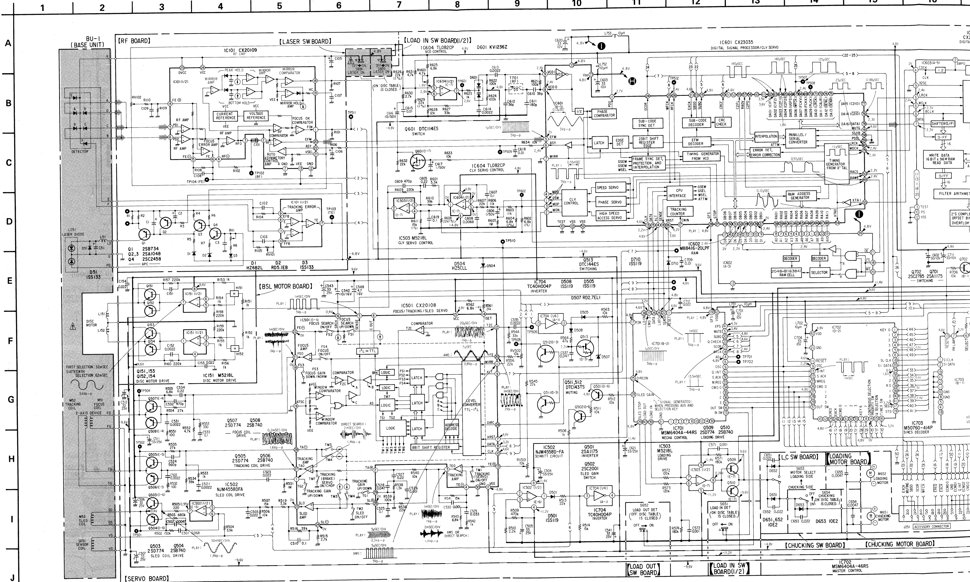
5-3. SCHEMATIC DIAGRAM — CDP502ES (AEP, UK model), CDP620ES (US model) — • See page 66 for notes.
