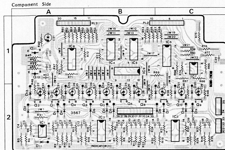
2-2. F-3567 Spectrum Analyzer Circuit Board (Stock No. 00648901)
