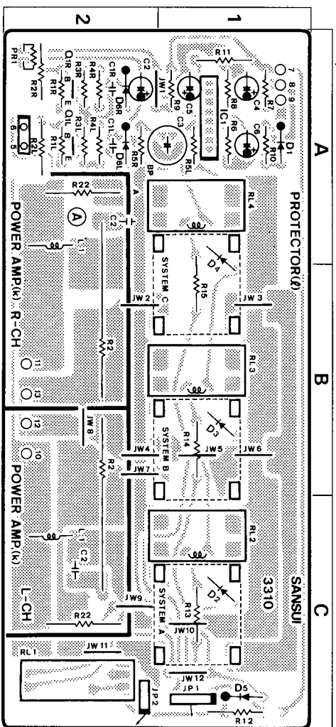
5-8. F-3310 Protector Circuit Board (Stock No. 00613601 = 9900Z/00619001 = 8900ZDB)
