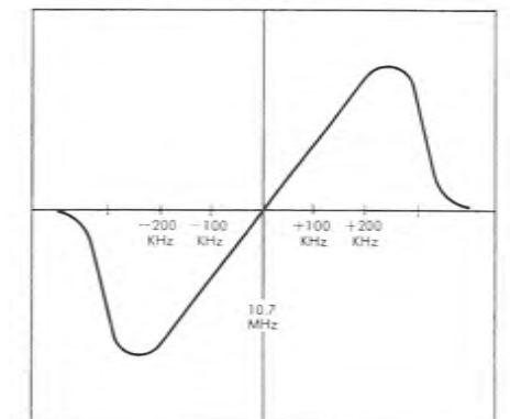
FM DISCRIMINATOR WAVE FORM
