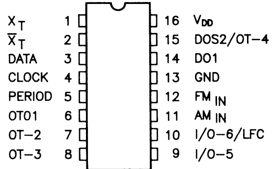
TC9216P BLOCK DIAGRAM
