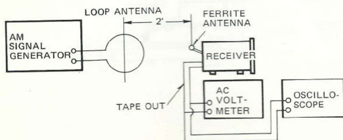
Fig. 1 AM ALIGNMENT CONNECTION
