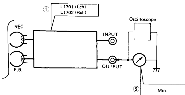
Fig. 5-11 Bias trap adjustment
