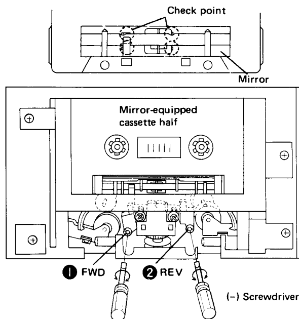
Fig. 4-4 Tape transport adjustment
