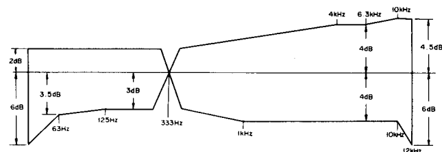
Fig. 5-16 Frequency response
