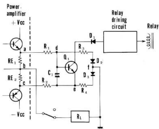
Fig. 17 Over-current and Overload Detection Circuit
