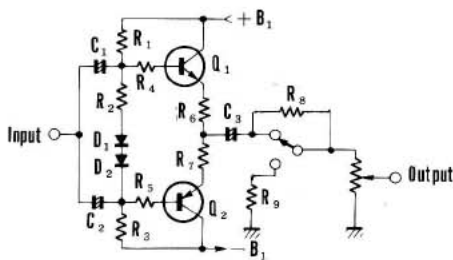
Fig. 7 Input Buffer Amplifier
