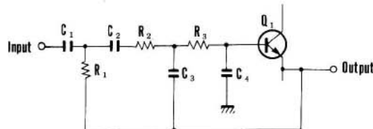
Fig. 12 Circuit Diagram of Filter Amplifier
