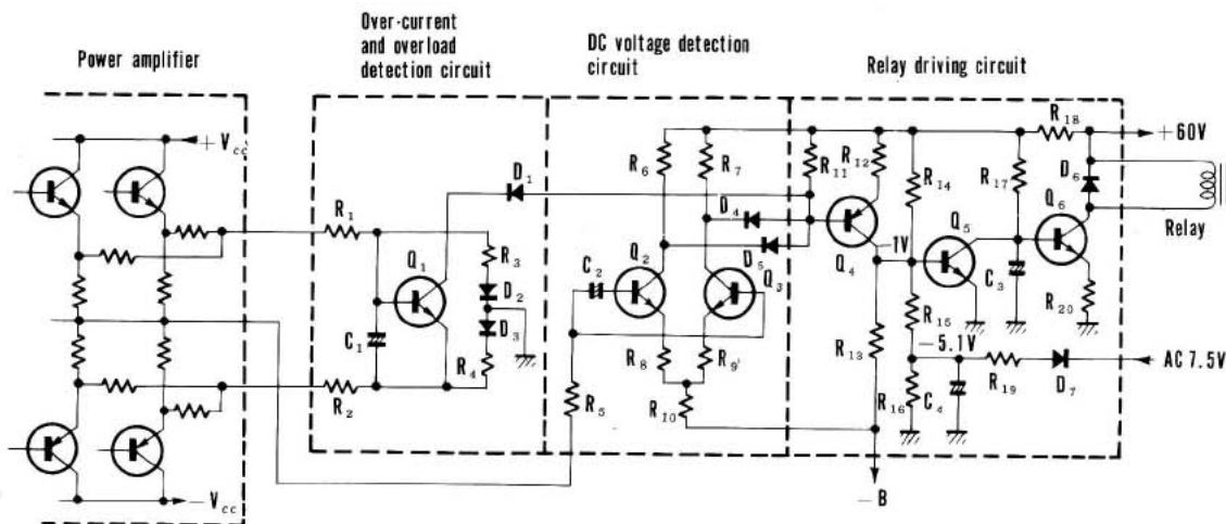
Fig. 15 Protection Circuit
