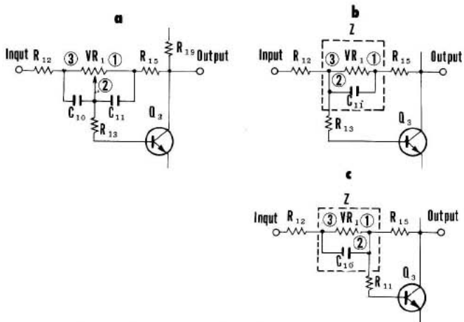
Fig. 10 Equivalent Circuit High Frequency Operation of Bass Boost and Cut
