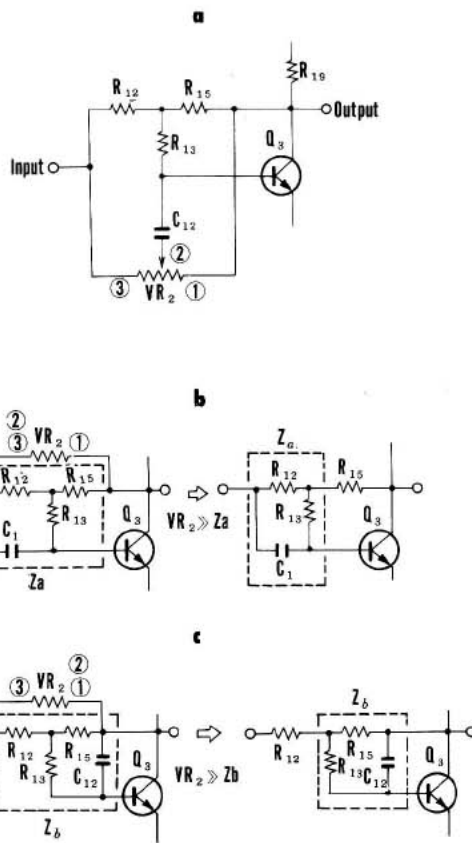
Fig. 11 Equivalent Circuit of Trouble Boost and Cut
