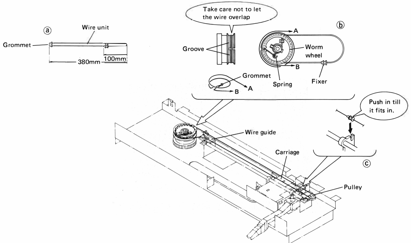
Fig. 6-4 Wire Replacement
