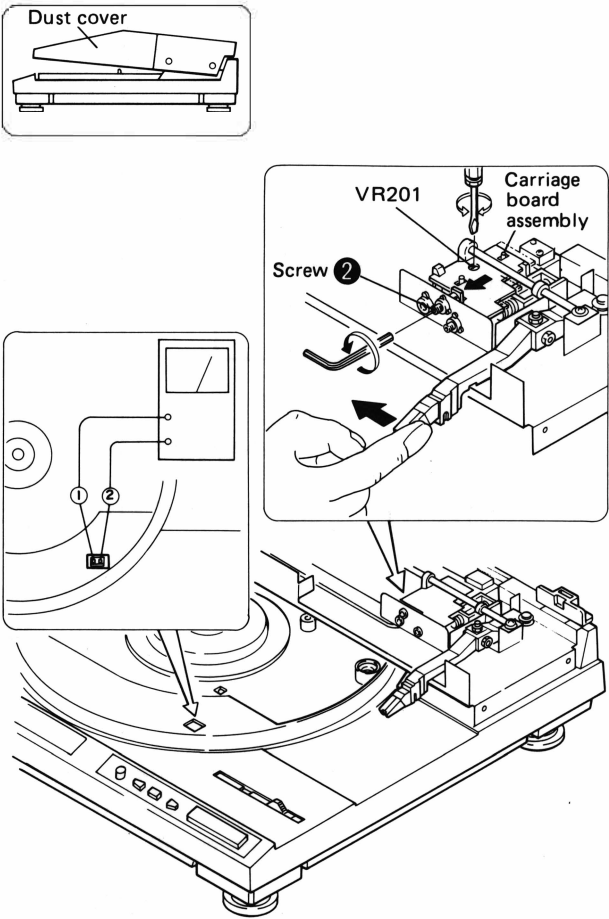
Fig. 13-2 Tracking Sensor Gain and Offset Adjustment
