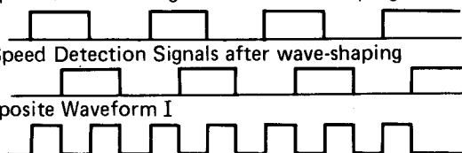
S1 Speed Detection Signals after wave-shaping
