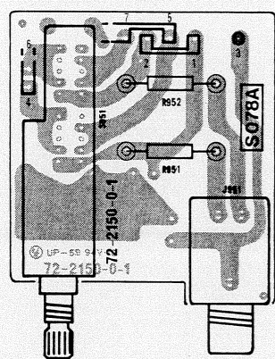
SPEAKER SWITCH PCB
