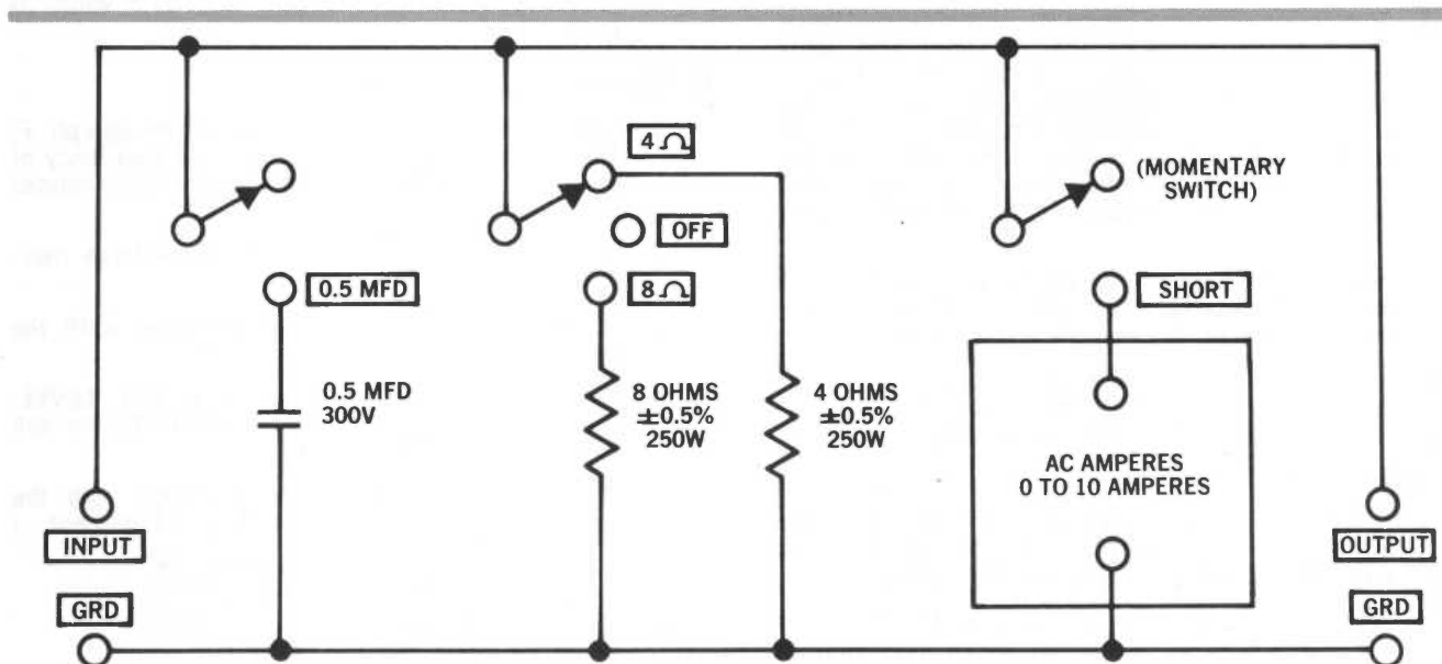
Figure 9. Amplifier Output Load Box, Schematic Diagram.
