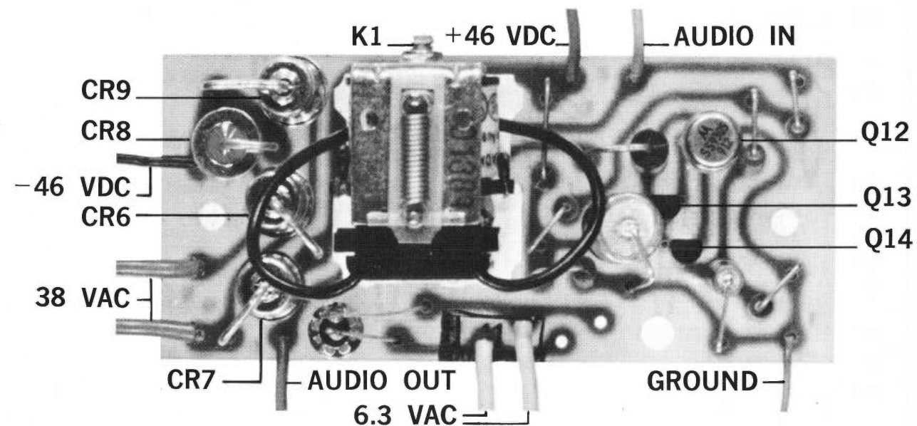
Figure 13. Relay Board.
