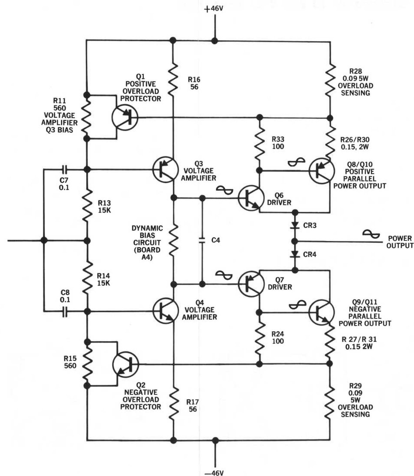
Figure 5. Amplifier Protection Circuit.
