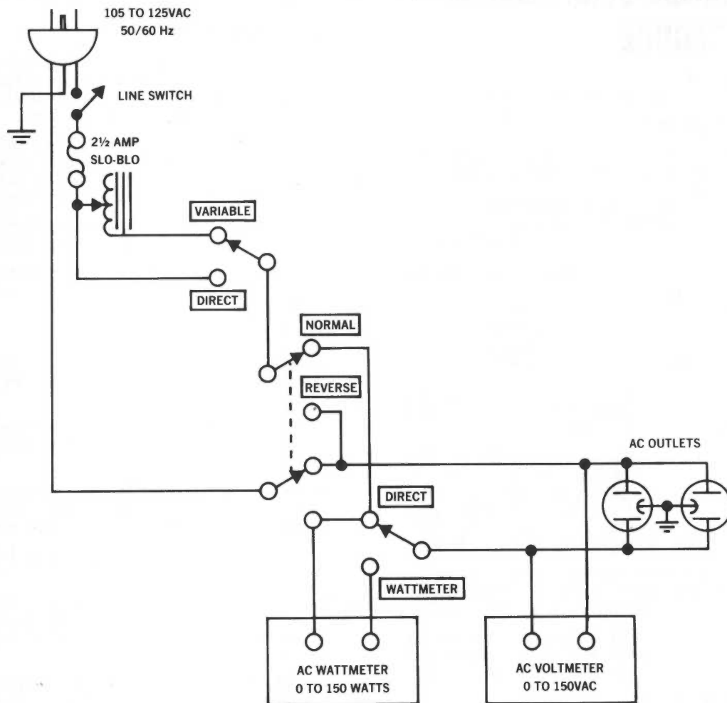
Figure 8. AC Power Control Box, Schematic Diagram.
