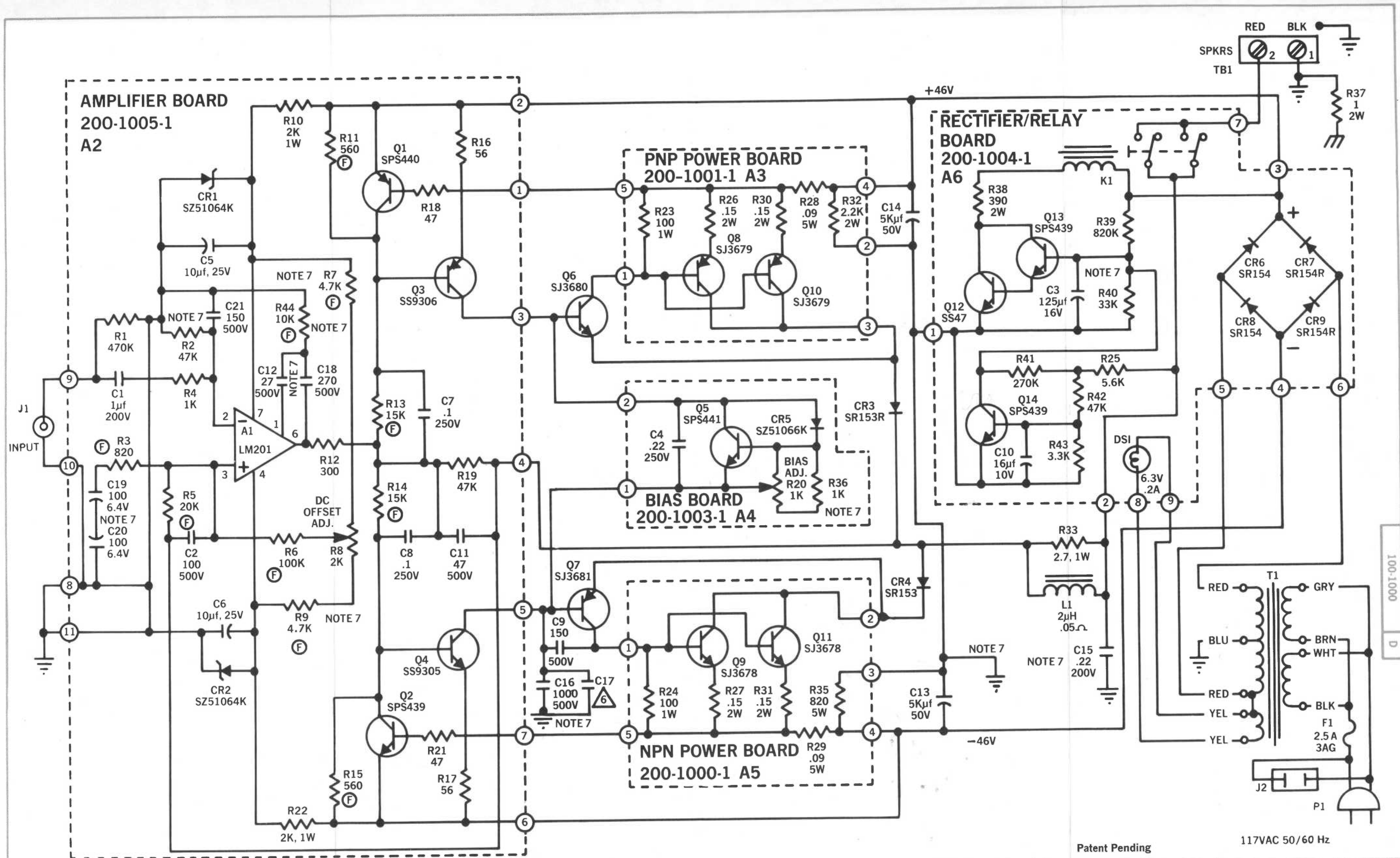
Figure 14. Marantz Model 16 Power Amplifier, Schematic Diagram.
