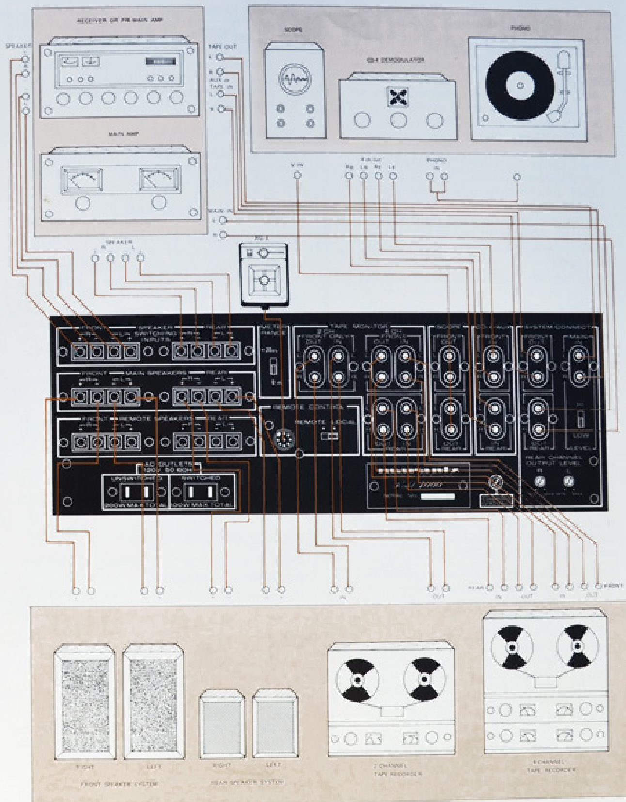
Figure 2. Connection Diagram
