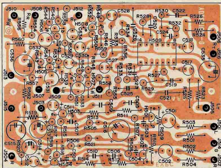
Figure 8. Phono Amplifier and SQ Decoder Assembly P500 Component Locations
