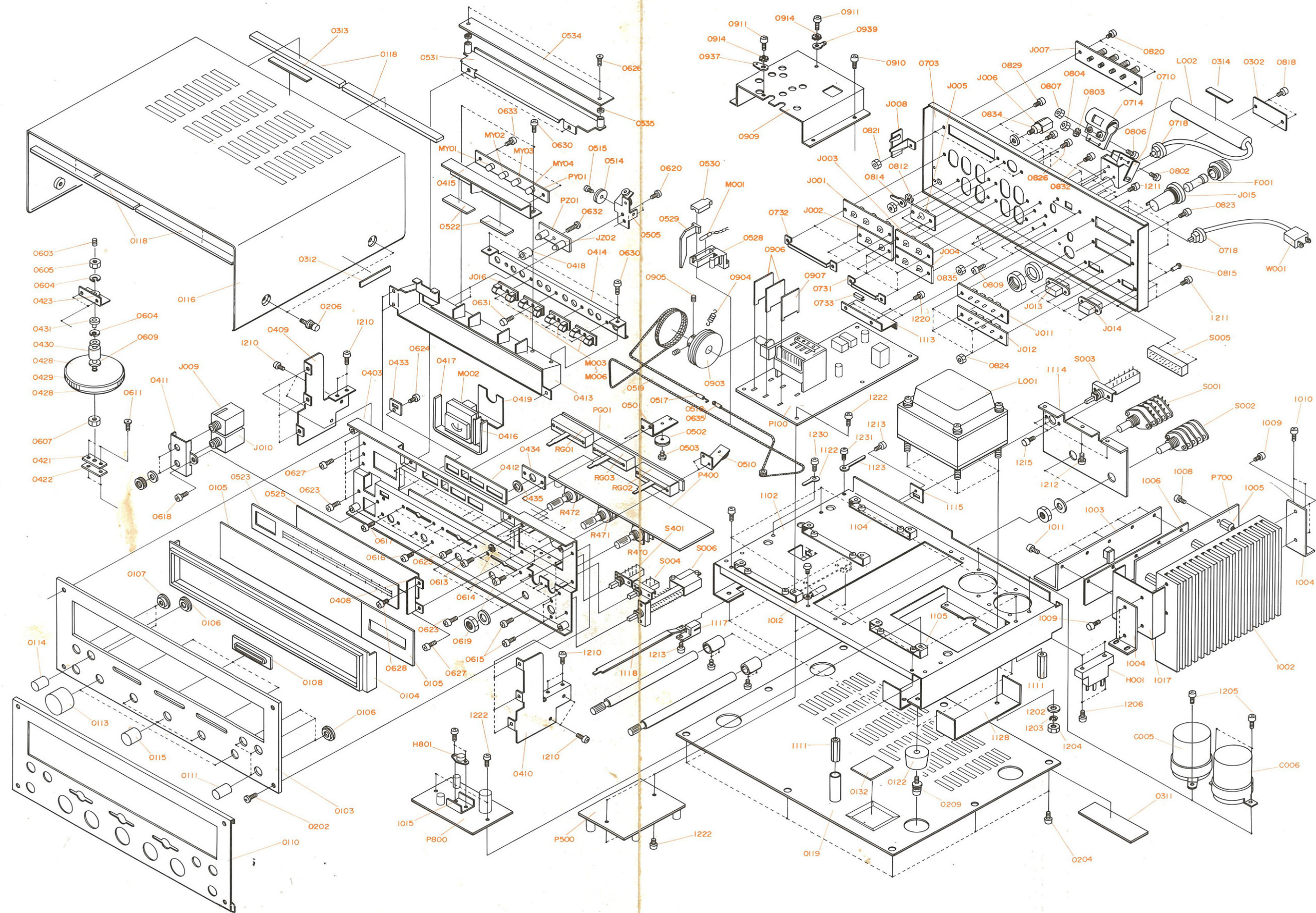
Figure 14. Exploded Mechanical Diagram
