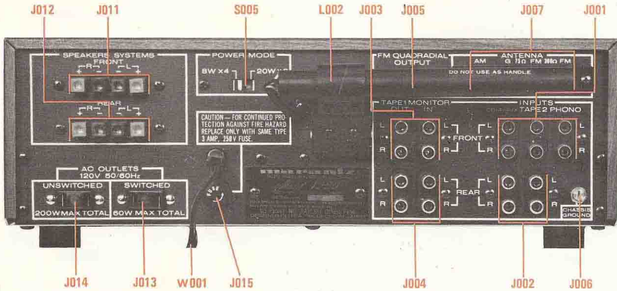
Figure 4. Rear Panel Adjustment and Component Locations
