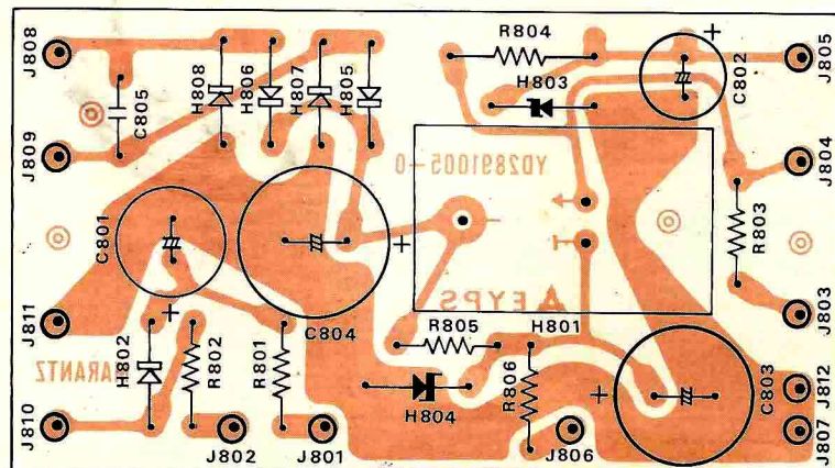
Figure 10. Power Supply Unit Assembly P800 Component Locations
