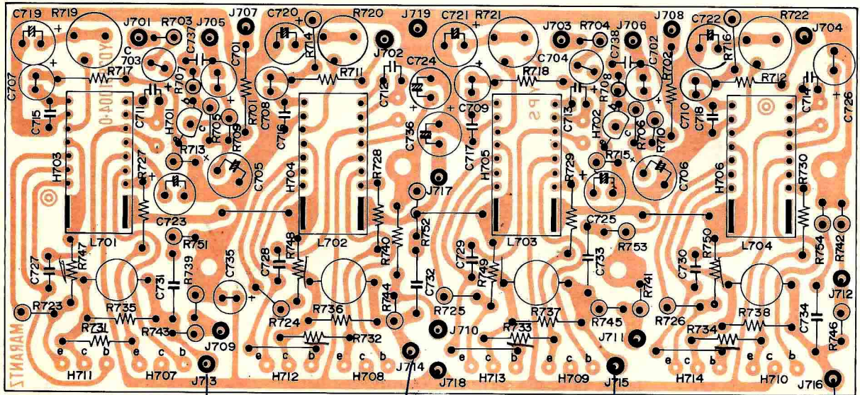
Figure 9. Power Amplifier Assembly P700 Component Locations
