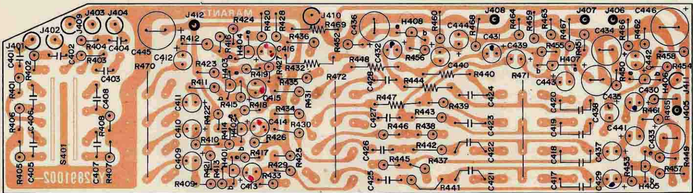
Figure 7. Tone Amplifier and Loudness Assembly P400 Component Locations
