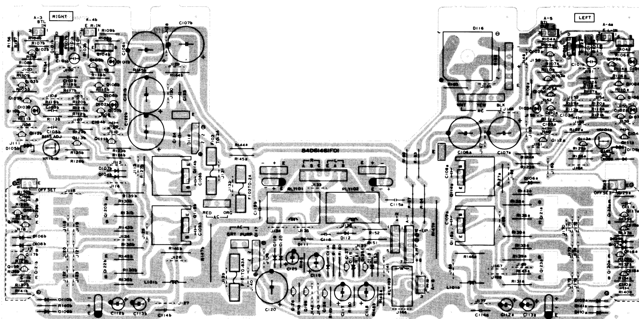
Main PCB
