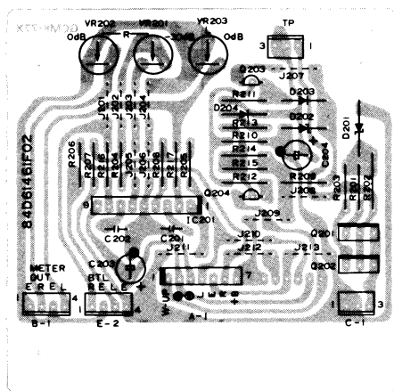
ACC PCB
