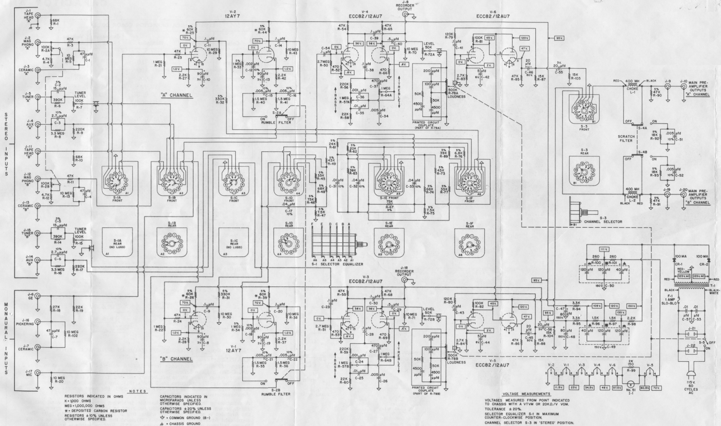
FIGURE 17. SCHEMATIC DIAGRAM
