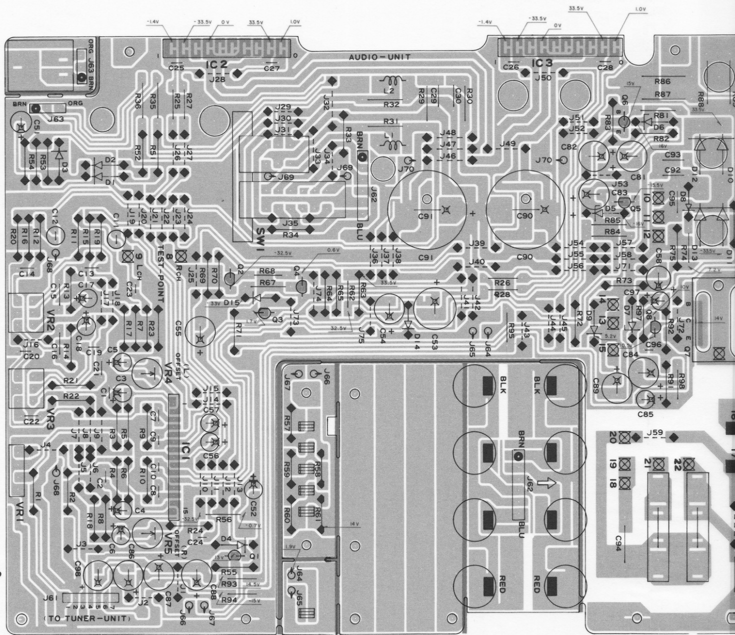
AUDIO AMP (X09-1530-10, 51, 81, X09-1532-71, 72) Component side view
