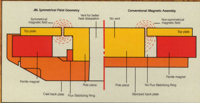
As this frequency driver cross section demonstrates, JBL's unique Symmetrical Field Geometry (SFG), shown on the left, dramatically reduces the second harmonic distortion found in conventional drivers, shown on the right, thereby optimizing bass performance.
