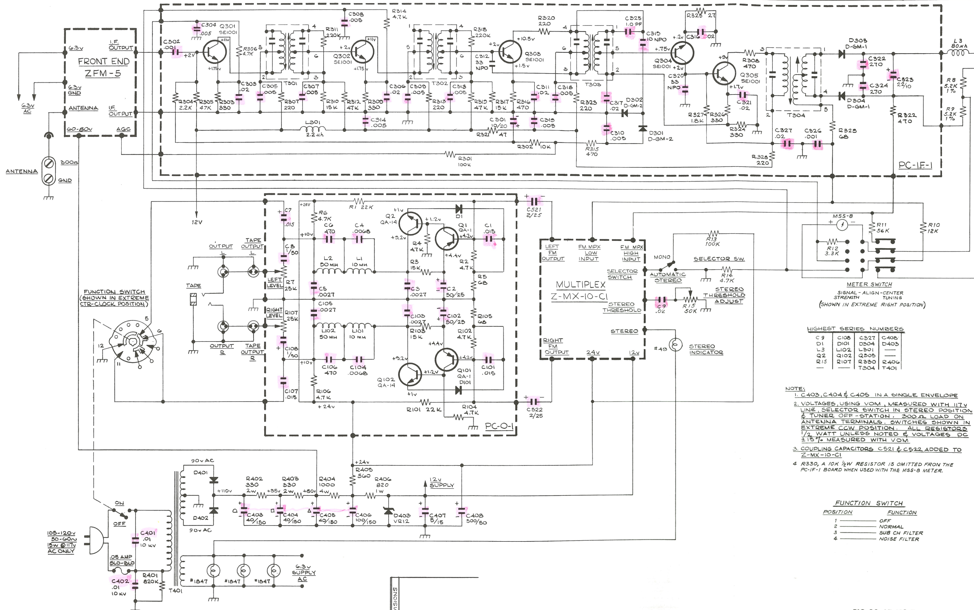
FIG. 22 LT-112 Tuner
