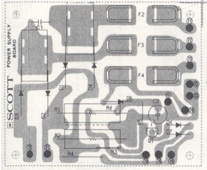
PSPW033COX, Power Supply
