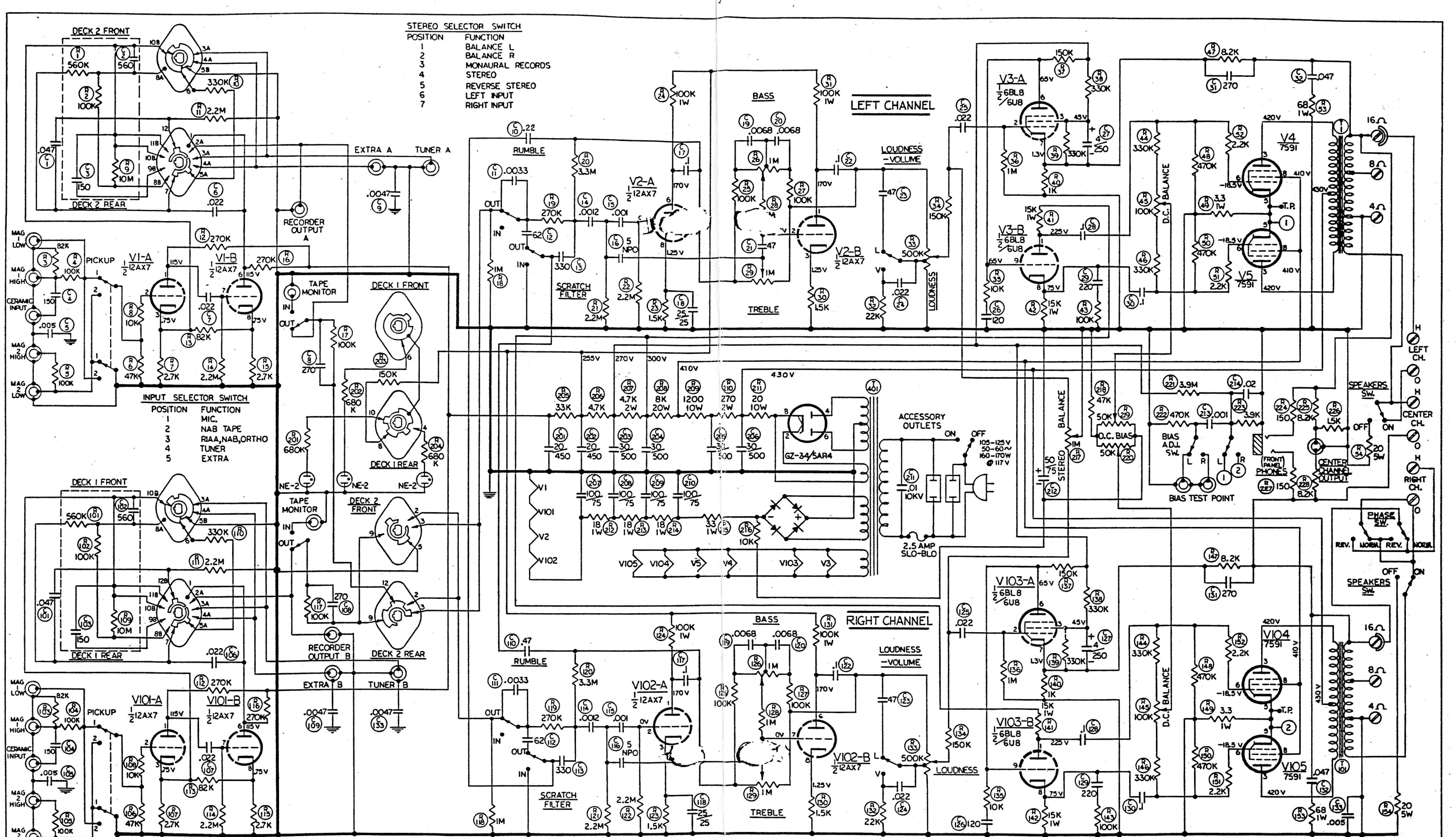
TYPE 299D STEREO AMPLIFIER
