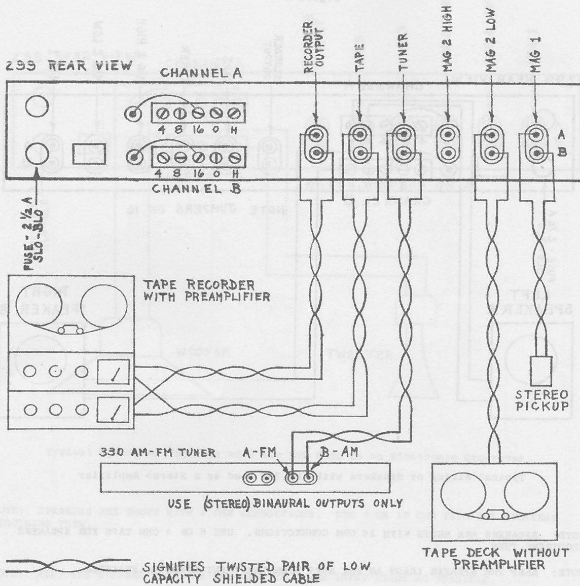
Typical Wiring of Inputs of the Type 299 Complete Stereo Amplifier
