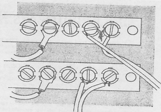
Touching wires at speaker terminals, in upper strip, short out the signal. Lower strip shows neat, trouble-free connection.
