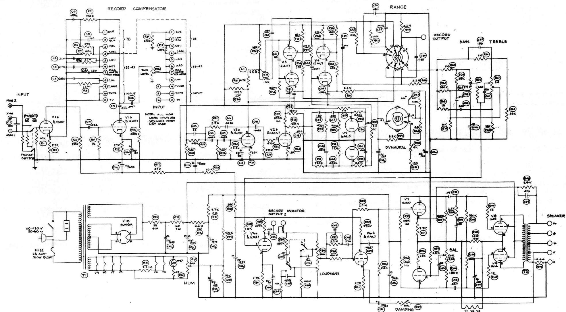
210-D DYNAURAL AMPLIFIER
