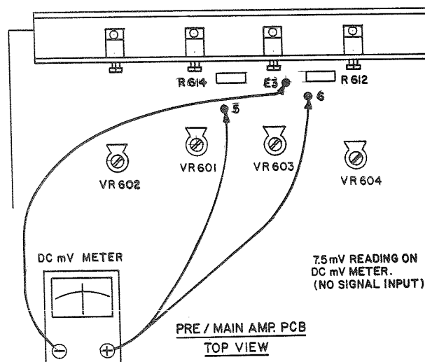
FIG. 2 IDLING CURRENT ADJUSTMENT HOOK-UP
