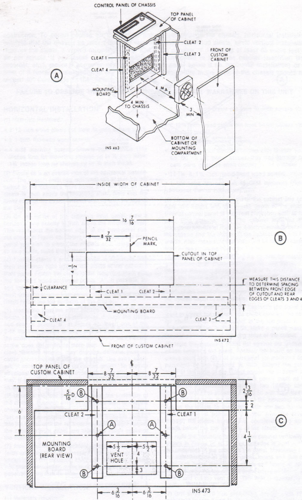
Figure 5. Vertical Installation
