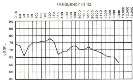
Figure 1. Typical Sound System Response Curve Before Equalization
