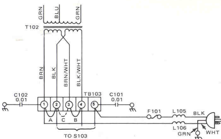
Figure 4. Converting to 240V, 50/60 Hz Power
