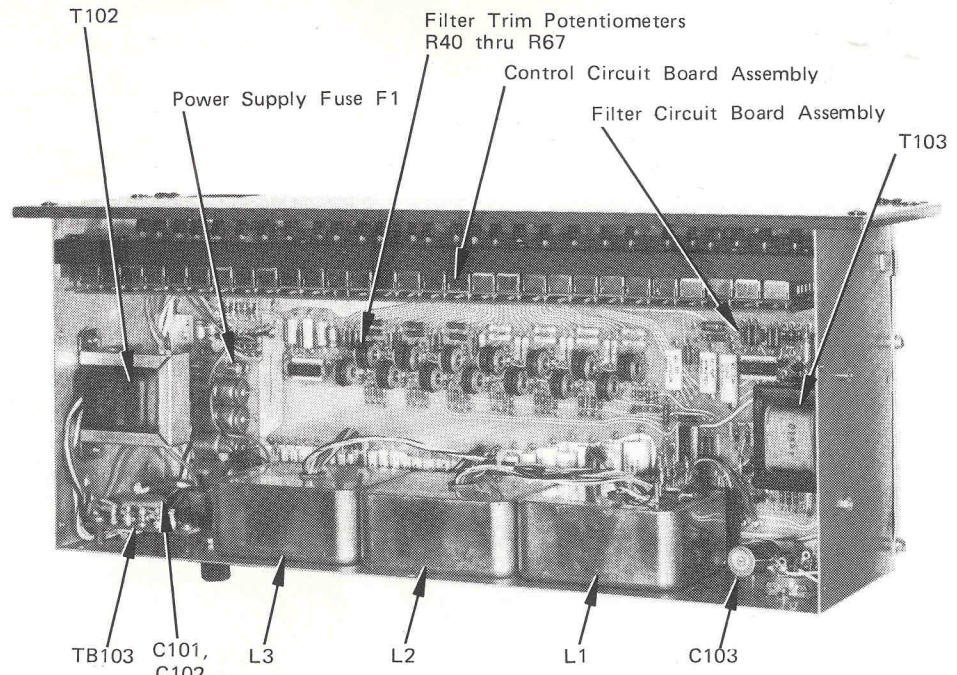
Figure 7. Internal View of 1650 Active Equalizer
