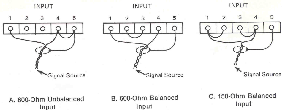
Figure 5. Input Connections at TB101
