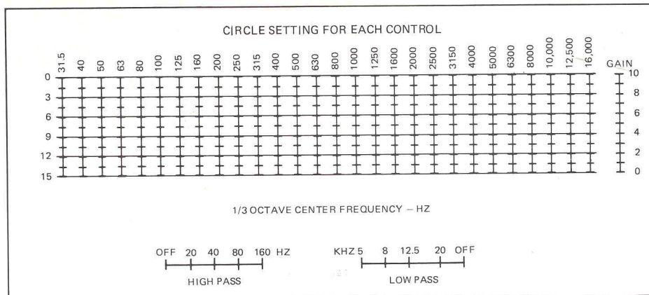
Figure 3. Control Settings Record
