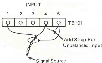
Figure 6. 15,000-Ohm Input Connections
