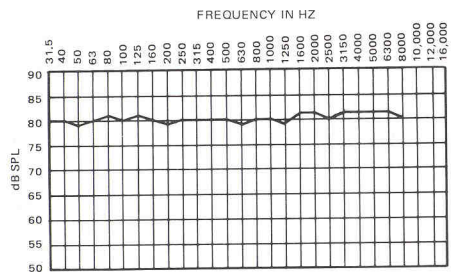
Figure 2. Typical Sound System Response Curve After Equalization
