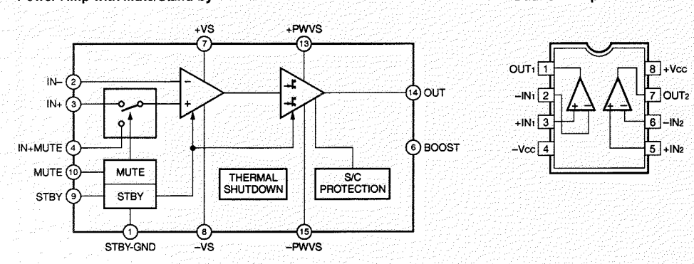
IC101, 102 : TDA7296 Power Amp with Mute/Stand-by
