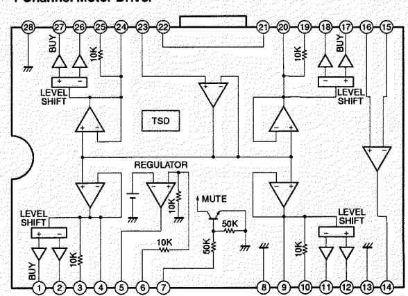
IC803 : KA9258D 4-Channel Motor Driver
