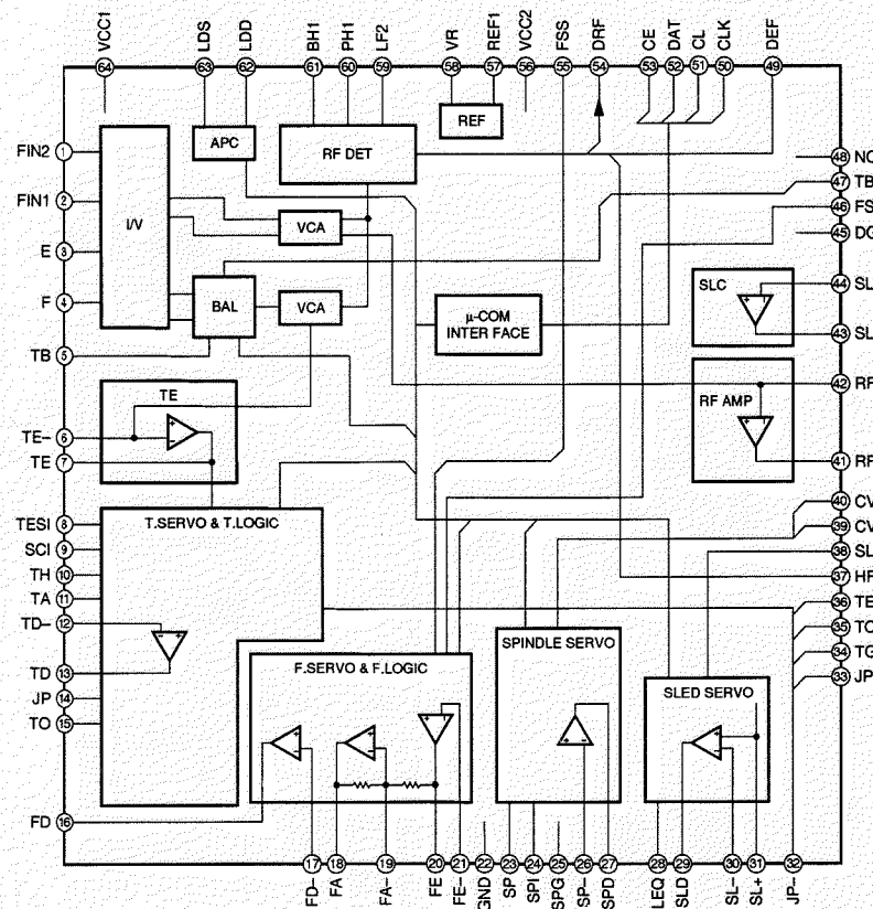
IC801 : LA9240M ASP
