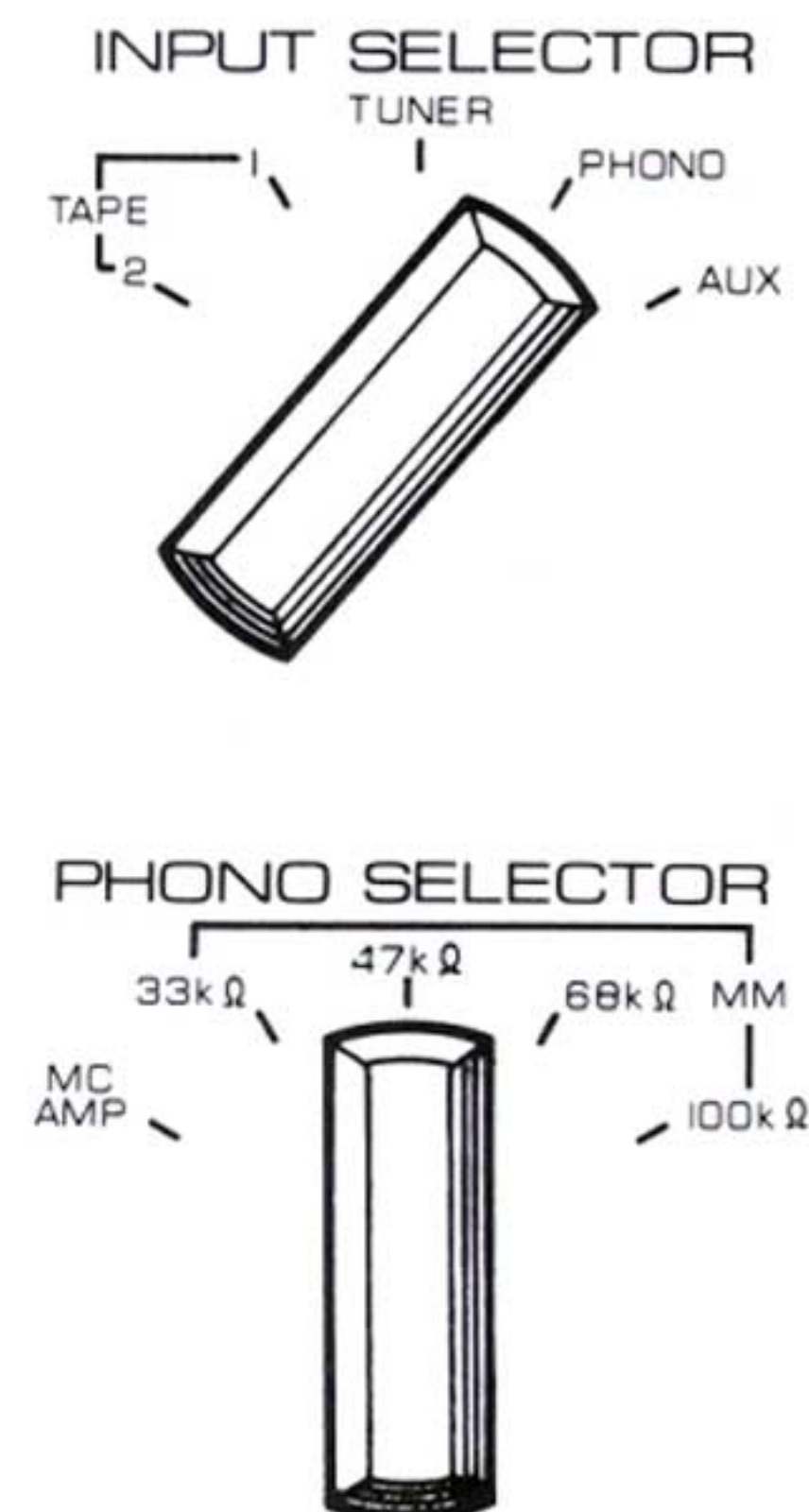
Fig. 15 INPUT SELECTOR and PHONO Selector Settings
