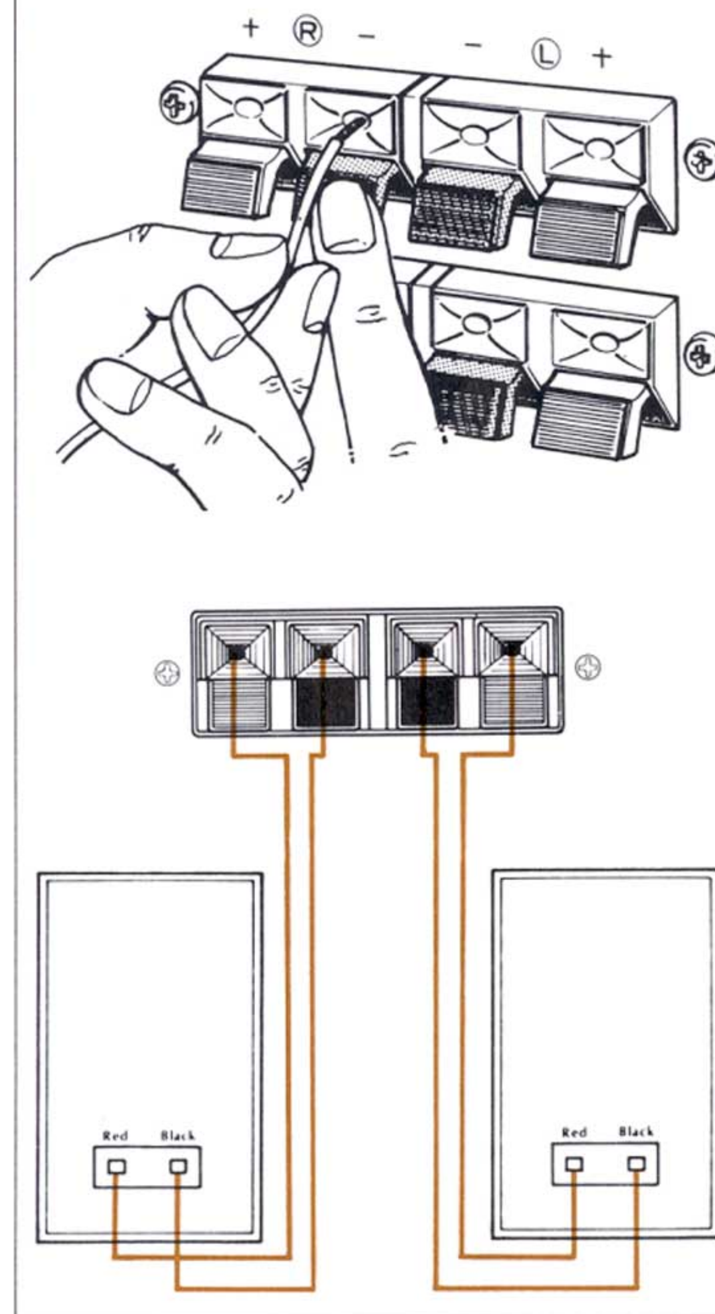
Speaker Connections
