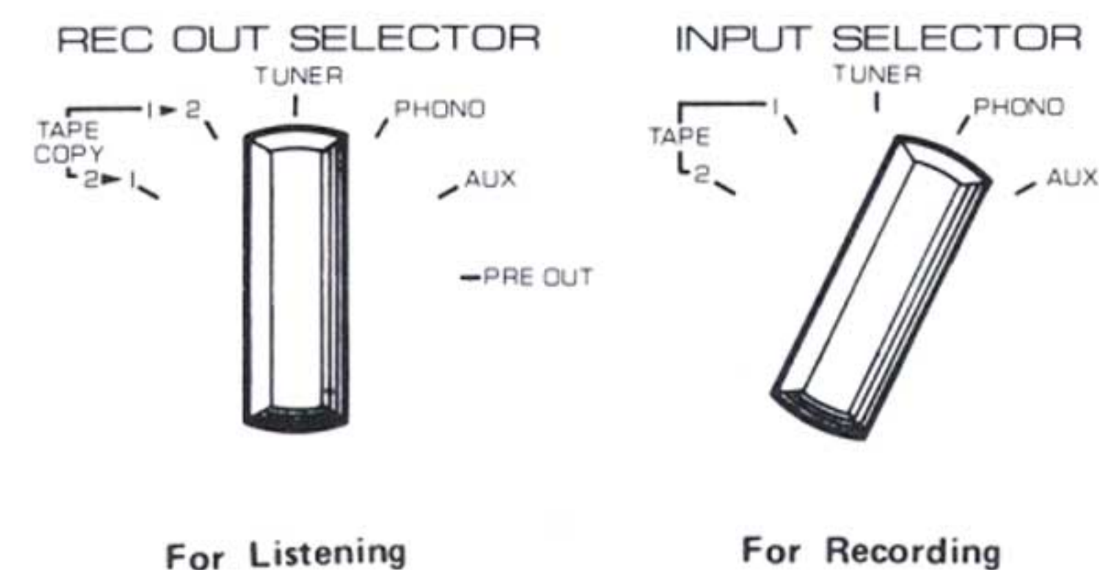
Fig. 18 Rec Out Selector & Input Selector Setting
