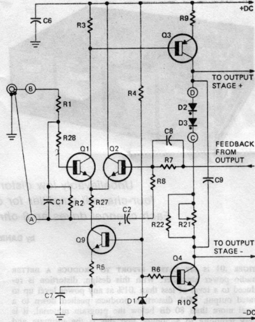
FIG. 3—CROSSOVER DISTORTION IS INHERENTLY LOW when current source replaces the driver bootstrap capacitor.
