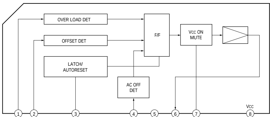
IC850 μPC1237HA
