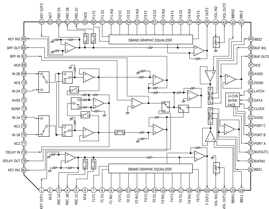
IC105 M62427FP-A
