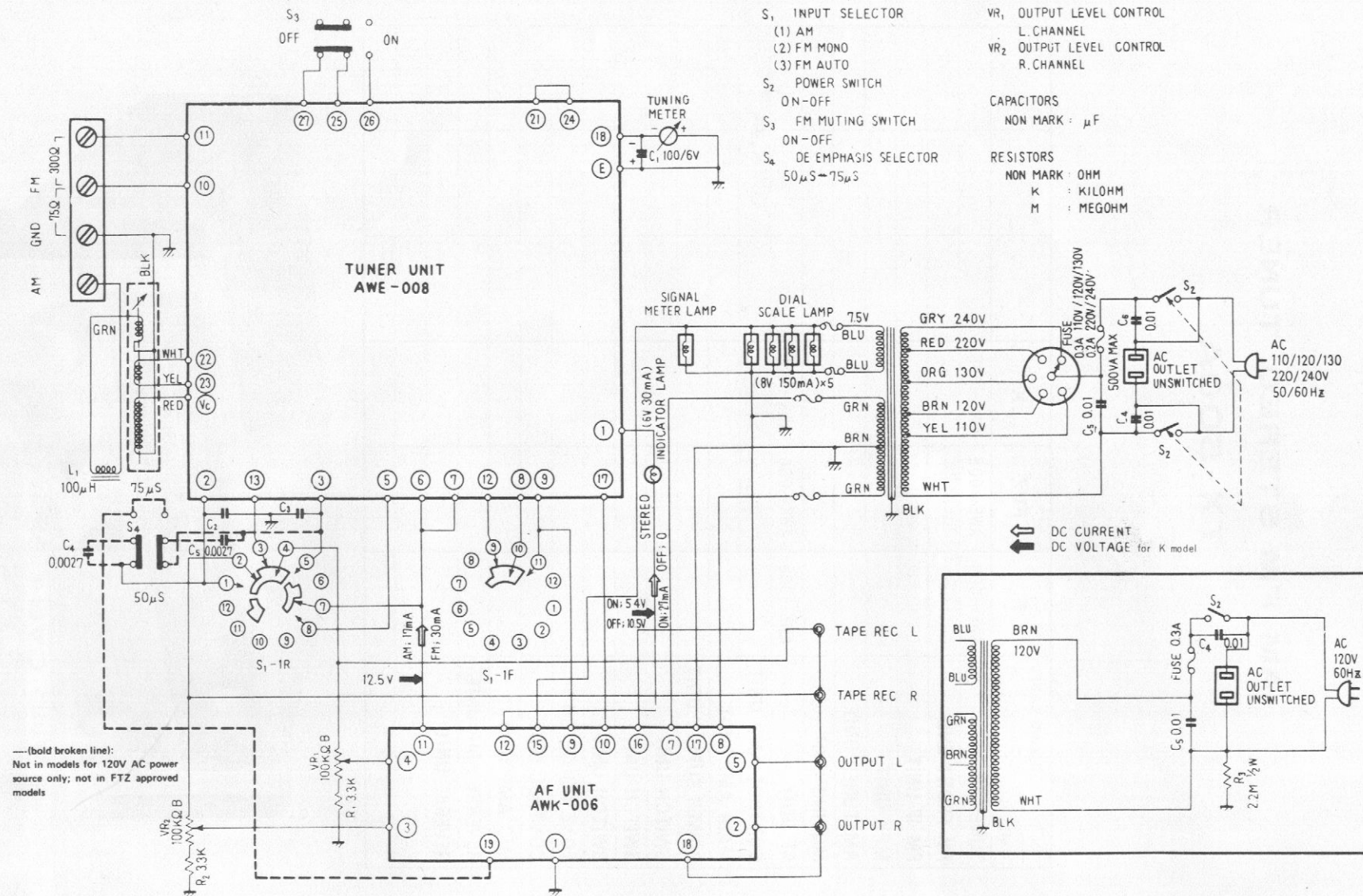
Power supply circuit for 120V AC only.
