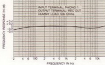
SX-07000: EQUALIZER RIAA DEVIATION
