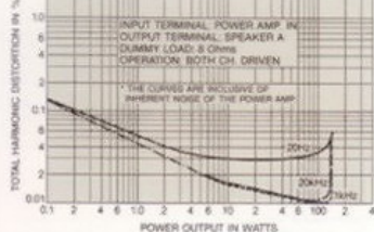
SX-07000: POWER OUTPUT vs. TOTAL HARMONIC DISTORTION
