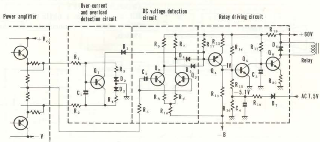
Fig. 9 Protection Circuit
