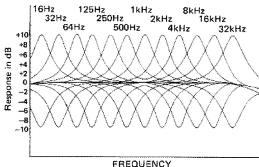
Fig. 1 Octave control variation curve
