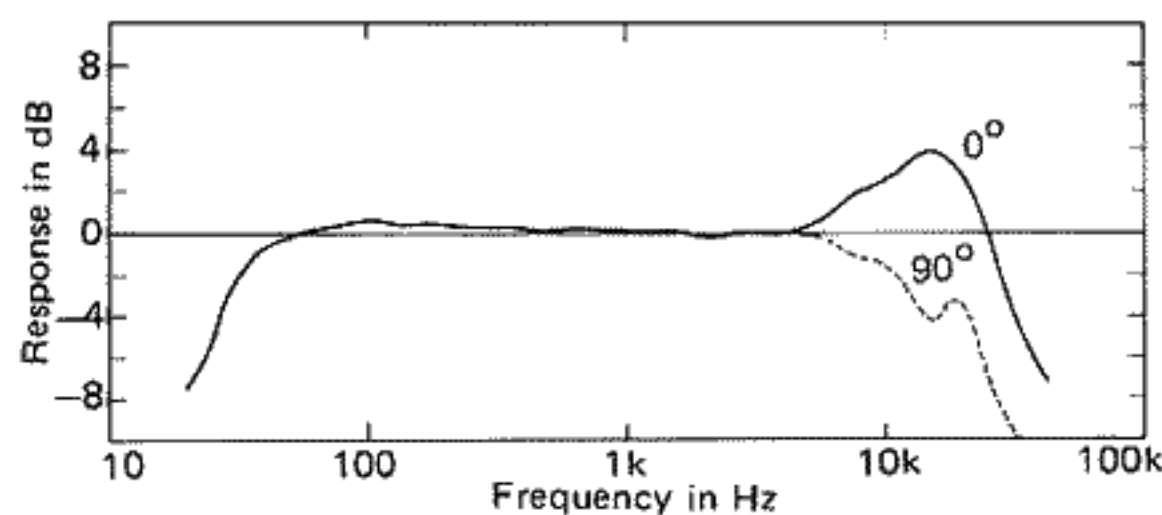
Fig. 12 Example of dynamic microphone response
