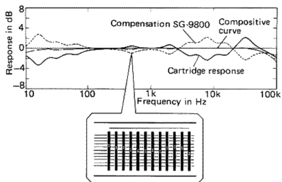
Fig. 10 MM cartridge high frequency compensation with SG-9800
