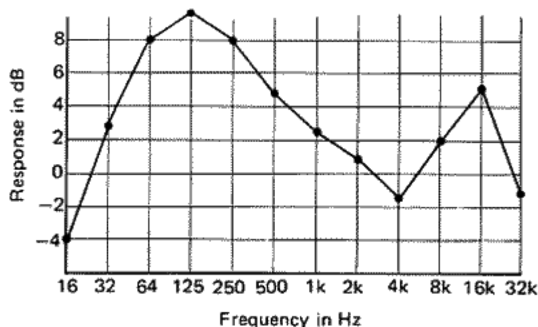
Fig. 14 Frequency line chart
