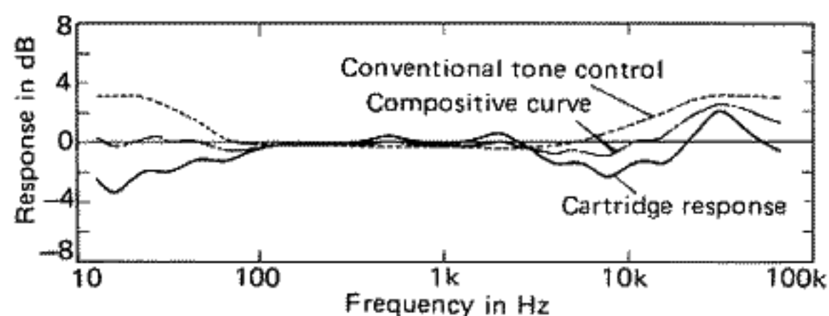
Fig. 9 MM cartridge high frequency compensation with conventional tone controls
