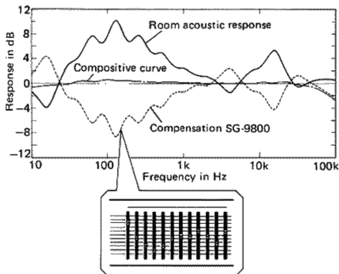
Fig. 13 Example of room acoustical response (transfer response)
