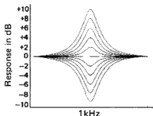
Fig. 2 1kHz Variation response
