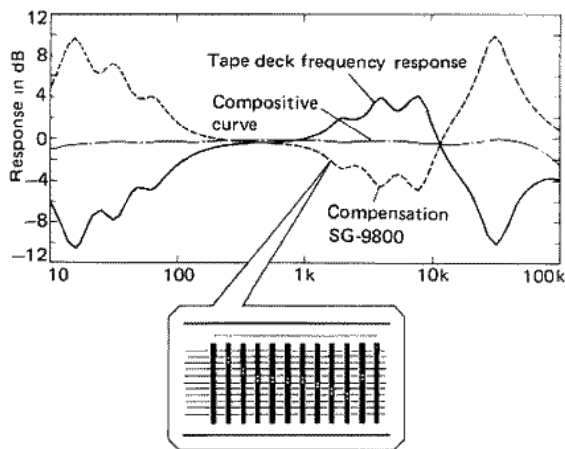
Fig. 11 Example of tape deck frequency response
