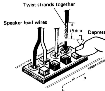
SPEAKER LEAD WIRE CONNECTION
