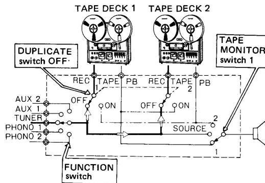
Tape recording: The input signal selected by the FUNCTION switch is always present at a fixed level at the TAPE 1 & 2 REC jacks. Monitoring can be performed at this time by setting the TAPE MONITOR switch to 1 or 2, according to the TAPE jacks being used for recording. Fig. 11
