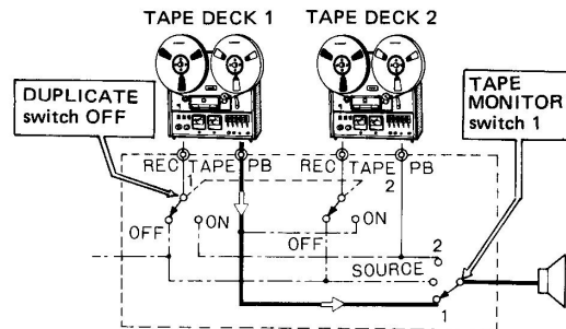
Tape playback: Playback signal enters TAPE 1 (or 2) PB jacks, passes through TAPE MONITOR switch 1 (or 2) and is heard from the speakers. Fig. 10
