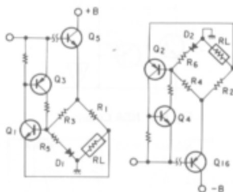
Fig. 5-5 Bridge Circuit
