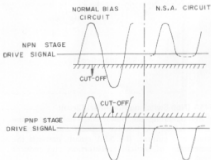
Fig. 5-9 Driving Signal of Power Stage
