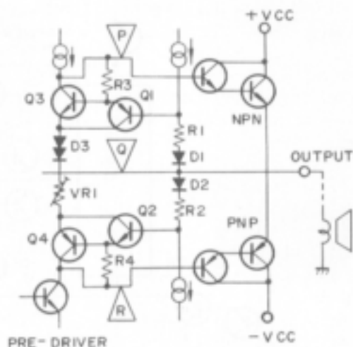
Fig. 5-7 NSA Circuit
