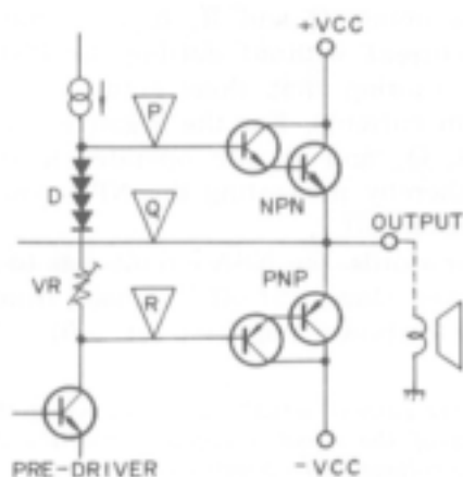
Fig. 5-6 Normal Power Stage
