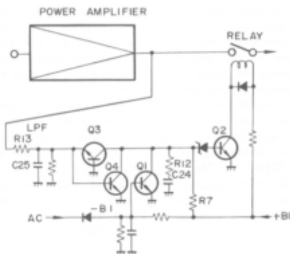
Fig. 5-11 Protection Circuit
