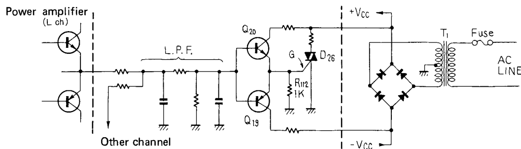
Fig. 5 Protection circuit
