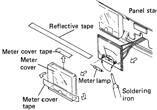
Fig. 9 Meter lamp replacement
