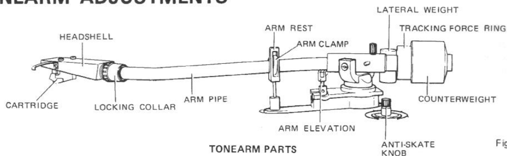
TONEARM PARTS
