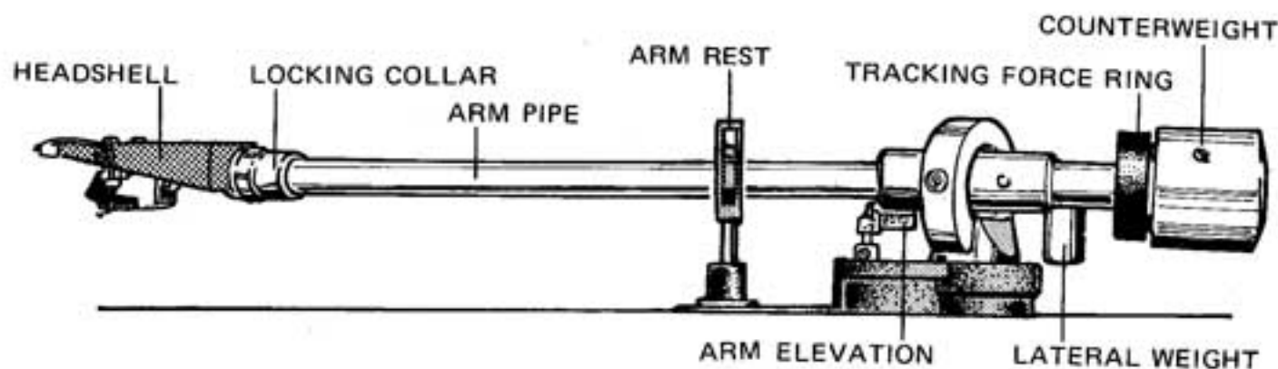
Tonearm Parts
