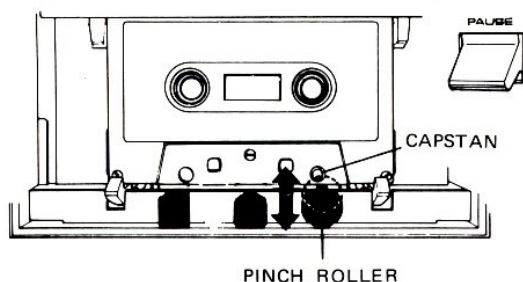
With PAUSE lever ON (depressed), pinch roller separates from capstan to stop only the tape motion. Motor (capstan) and amplifier continue to operate. Fig. 5
