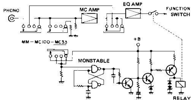
Fig. 4-3 Phono system muting circuit
