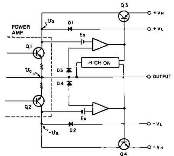
Fig. 4-8 Basic circuitry
