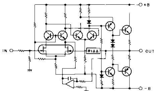
Fig. 4-2 Equalizer amplifier
