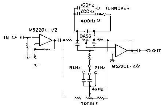
Fig. 4-4 Tone control
