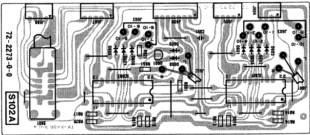
SELECTOR P.C.B. ASS'Y (S102A)
