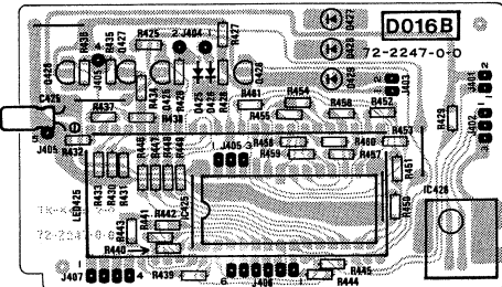
LED DISPLAY ASS'Y (D016B)
