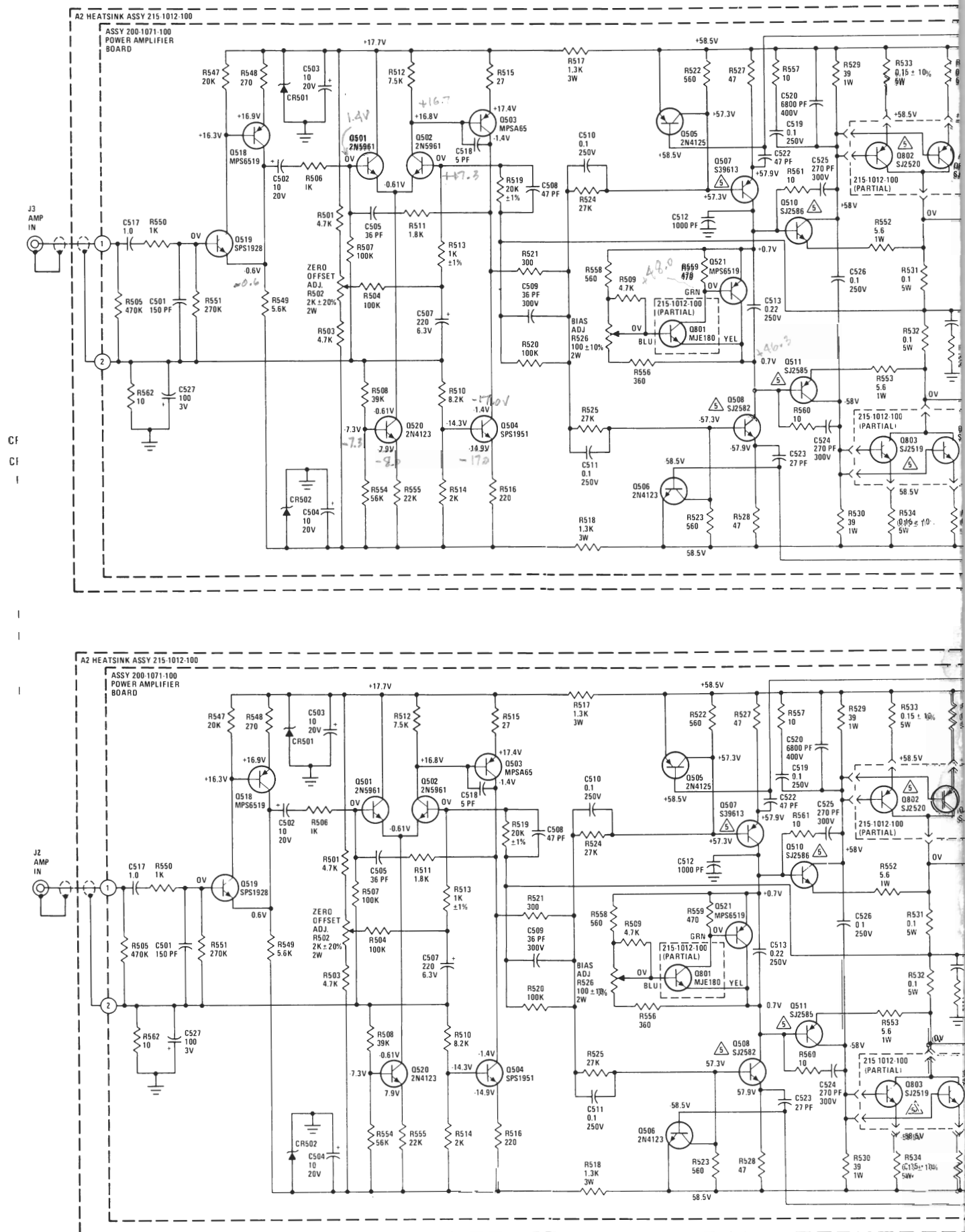
Figure 10. Model 250 Schematic
