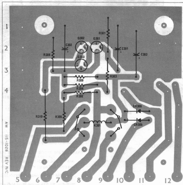
CIRCUIT SIDE
