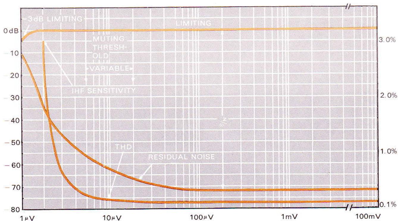
Figure 13. FM Characteristics
