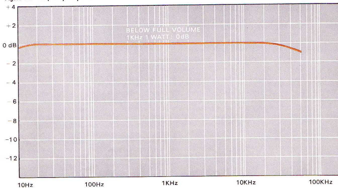
Figure 16. Frequency Response
