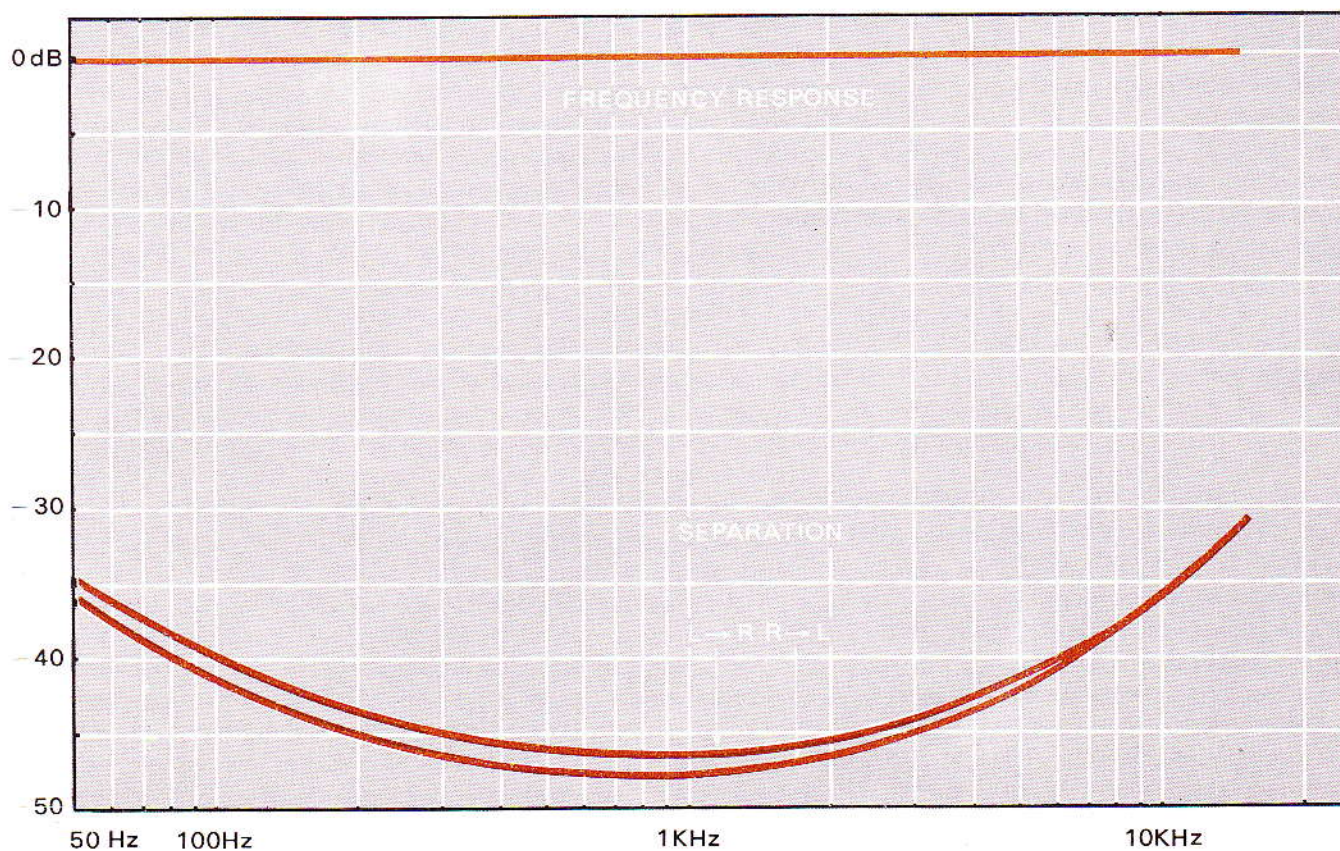
Figure 14. Stereo Separation
