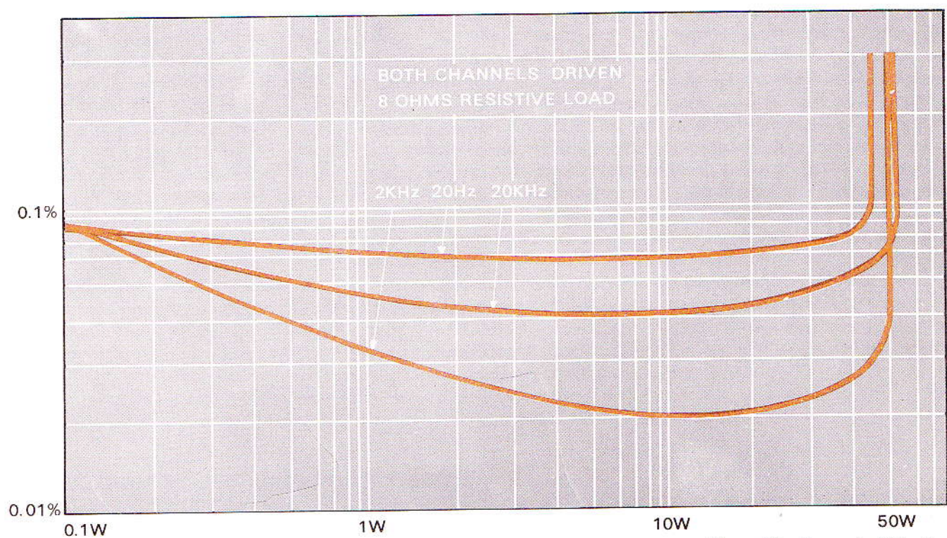
Figure 15. Harmonic Distortion
