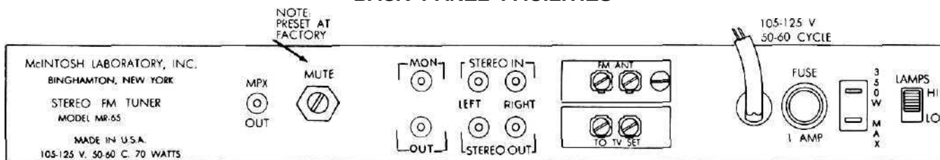
Fig. 9—Rear of chassis showing jacks, terminals, and adjustments.
