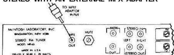
Fig. 16—Connections for an external MPX adapter.
