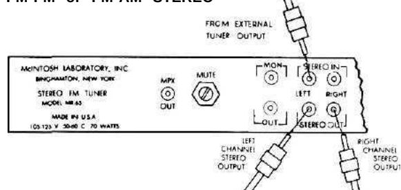
Fig. 17—Connection for external tuner for stereo.
