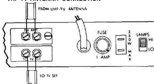
Fig. 20—Connections for sharing a VHF-TV antenna.
