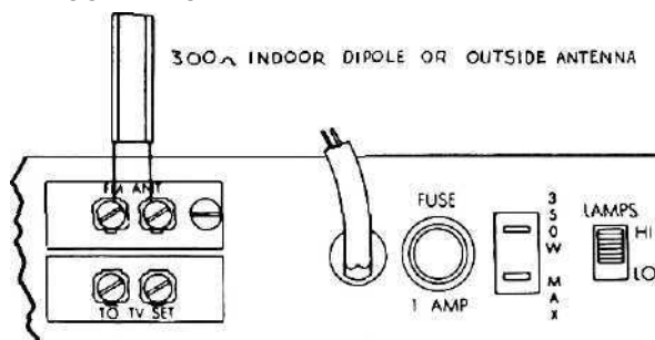
Fig. 18—Connection for 300 ohm antenna.
